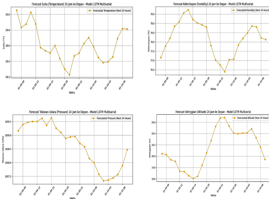
Gambar 4. Grafik hasil forecasting model LSTM multivariat
